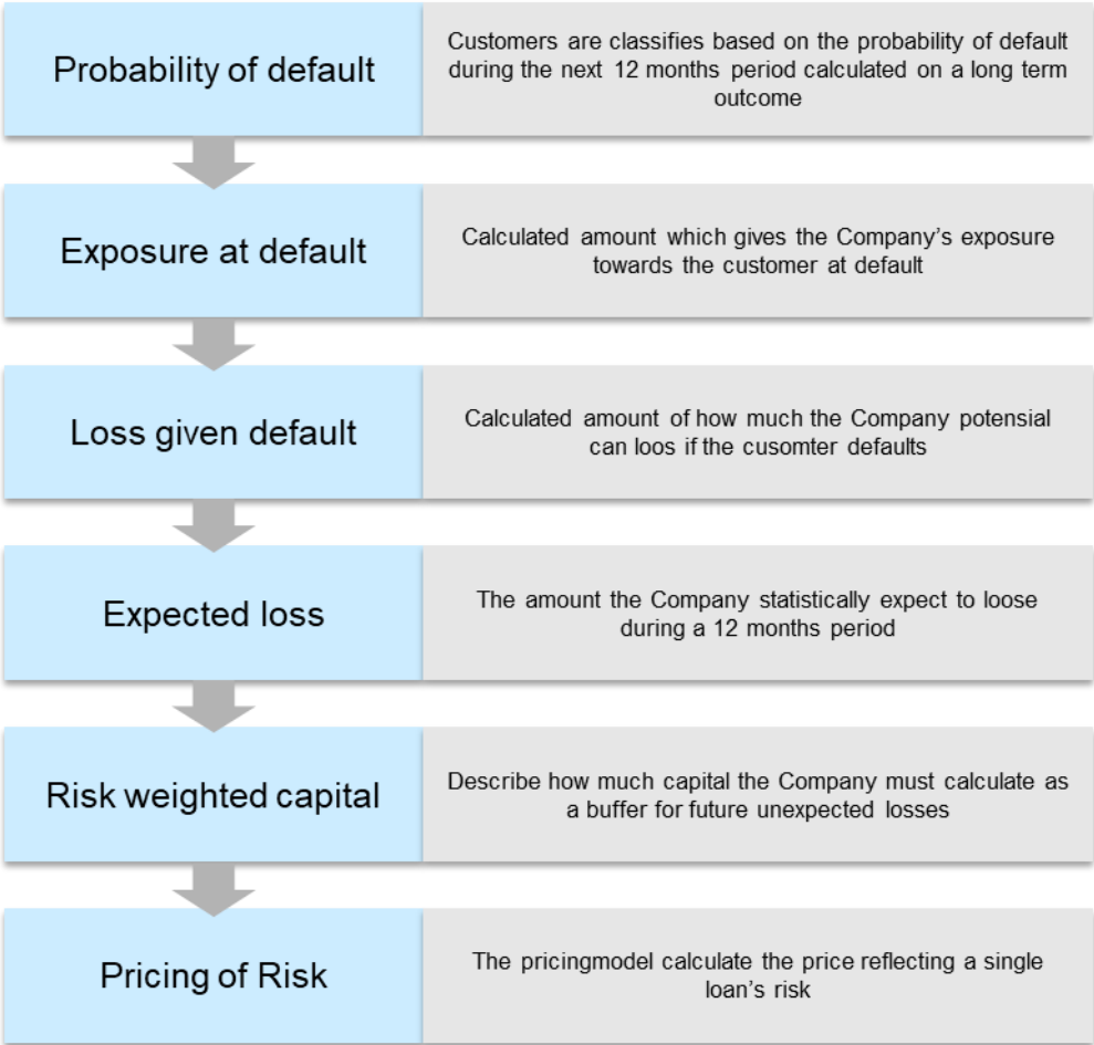
Figure 5: Riskclassification system
